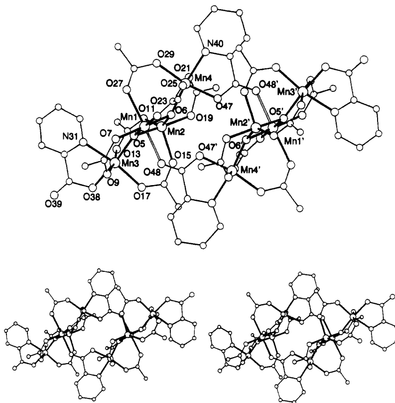
Figure 1. Labeled structure and stereoview of complex 2 . To avoid congestion, not all symmetry-equivalent atoms have been labeled. The \mu_3 -O atoms are O5, O5', O6, and O6'. Selected distances (Å): Mn1...Mn2, 2.876 (7); Mn1...Mn3, 3.450 (7); Mn1...Mn4, 3.309; Mn2...Mn3, 3.248 (7); Mn2...Mn4, 3.300 (7); Mn1-O5, 1.932 (19); Mn2-O5, 1.863 (20); Mn3-O5, 1.872 (19); Mn1-O6, 1.904 (20); Mn2-O6, 1.882 (20); Mn4-O6, 1.859 (19); Mn1-O48, 2.236 (19); Mn4-O47, 1.946 (20); Mn3-N31, 2.060 (25); Mn4-N40, 2.038 (23); Mn3-O38, 1.905 (20); Mn1-O7, 1.956 (23); Mn1-O23, 1.939 (23); Mn1-O27, 2.222 (21); Mn2-O11, 1.997 (21); Mn2-O15, 2.061 (20); Mn2-O19, 1.947 (21); Mn3-O9, 2.134 (20); Mn3-O13, 2.213 (23); Mn3-O17, 1.970 (20); Mn4-O21, 2.237 (23); Mn4-O25, 2.126 (20); Mn4-O29, 1.927 (20).
